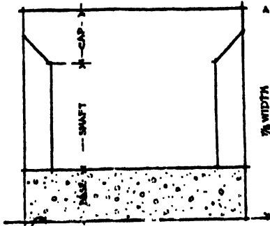
SUGGESTED SECTION OF FOUNDATION
